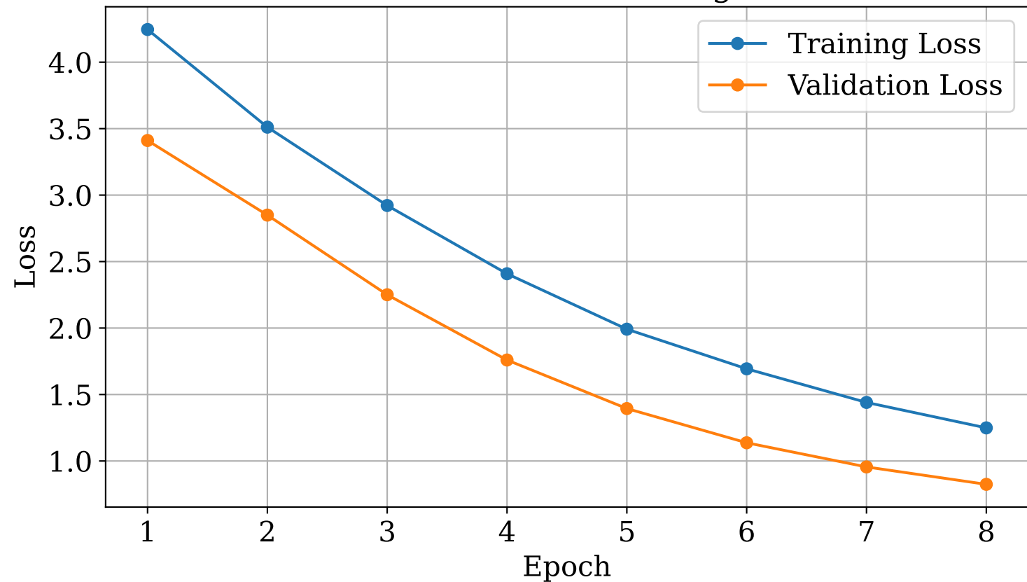
MobileNetV2 Fine-Tuning - Loss
